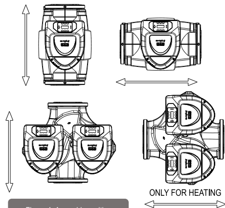
Figure 1: Assembly position
