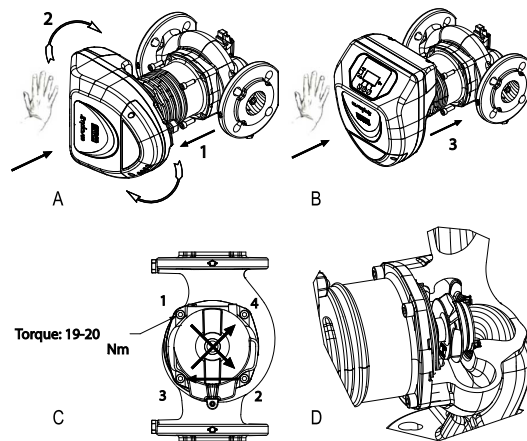
Figure 2: Instructions for motor head assembly
