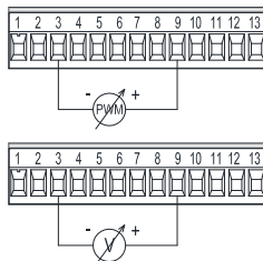
Figura 8: Pull-out 13-pole term Figura 8: Terminal de bomes extraible 13 polos:
